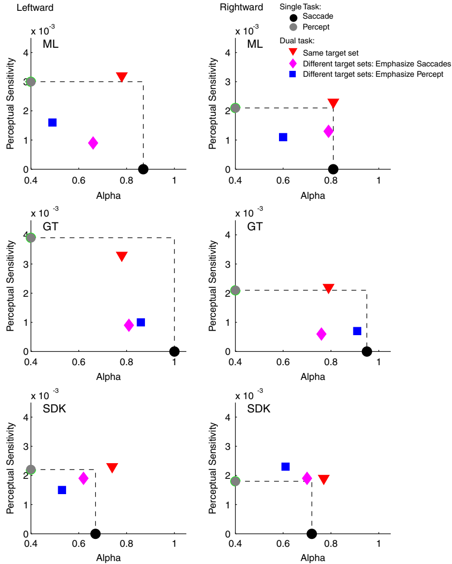
Fig. 6. Attentional operating characteristics. Saccadic performance (represented by the value of weighting parameter \alpha , Eq. (1)) vs. perceptual performance (represented by slope of the psychometric functions at the 50% point). Performance plotted along each axis comes from single-task (saccadic or perceptual) results. Intersection of single-task results (dashed line) is the independence point. Remaining data points show dual-task results (saccadic and perceptual task concurrently) when saccades and perceptual judgments were based on the same set of elements (triangle), or saccades and perceptual judgments were based on different sets of elements under instructions to give higher priority to the saccadic task (diamonds) or to the perceptual task (squares). Each datum point is based on approximately 100 observations.
