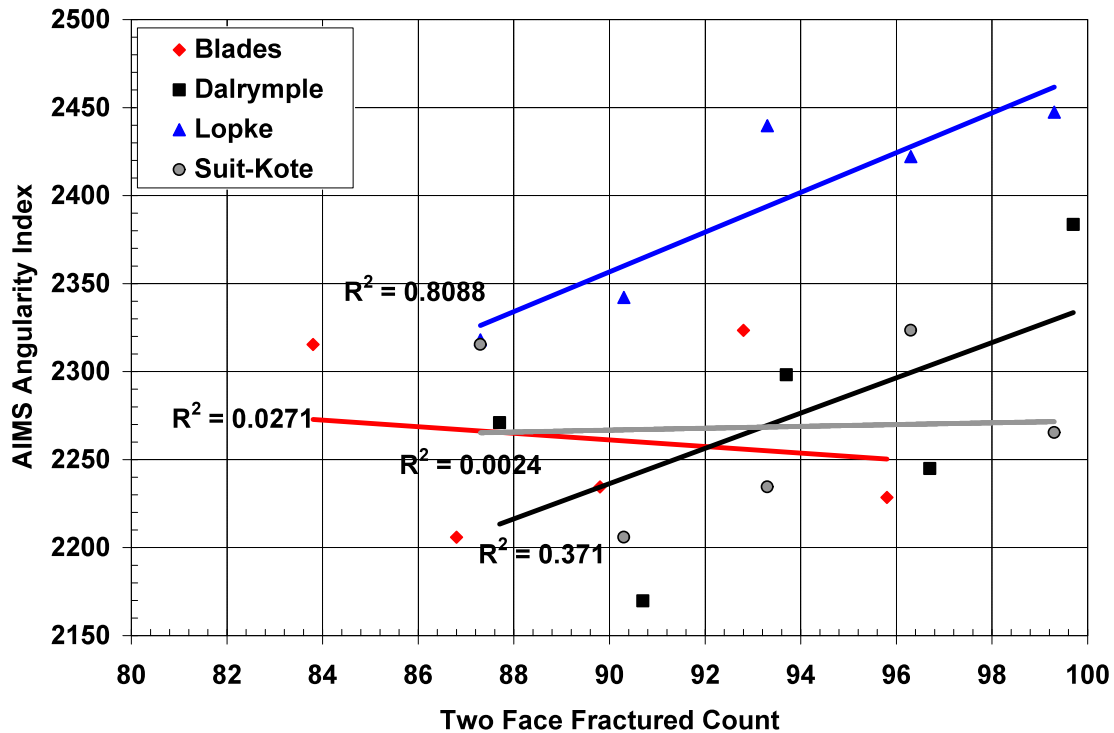
Figure 4.20 – Gravel Source Relationship Between AIMS Angularity Index and Two Face Fractured Count
