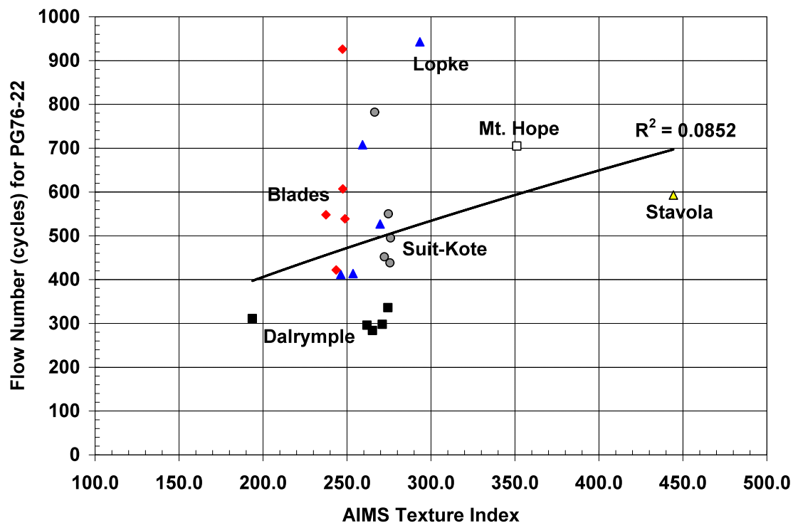
Figure 6.33 – AIMS Texture Index vs Flow Number for the PG76-22 Asphalt Binder
