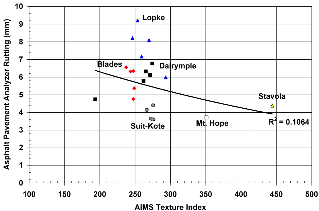
Figure 6.16 – Asphalt Pavement Analyzer Rutting for All Mixtures vs AIMS Texture Index – PG64-22 Asphalt Binder
