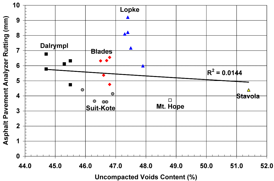
Figure 6.13 – Asphalt Pavement Analyzer Rutting for All Mixtures vs Uncompacted Voids Content – PG64-22 Asphalt Binder
