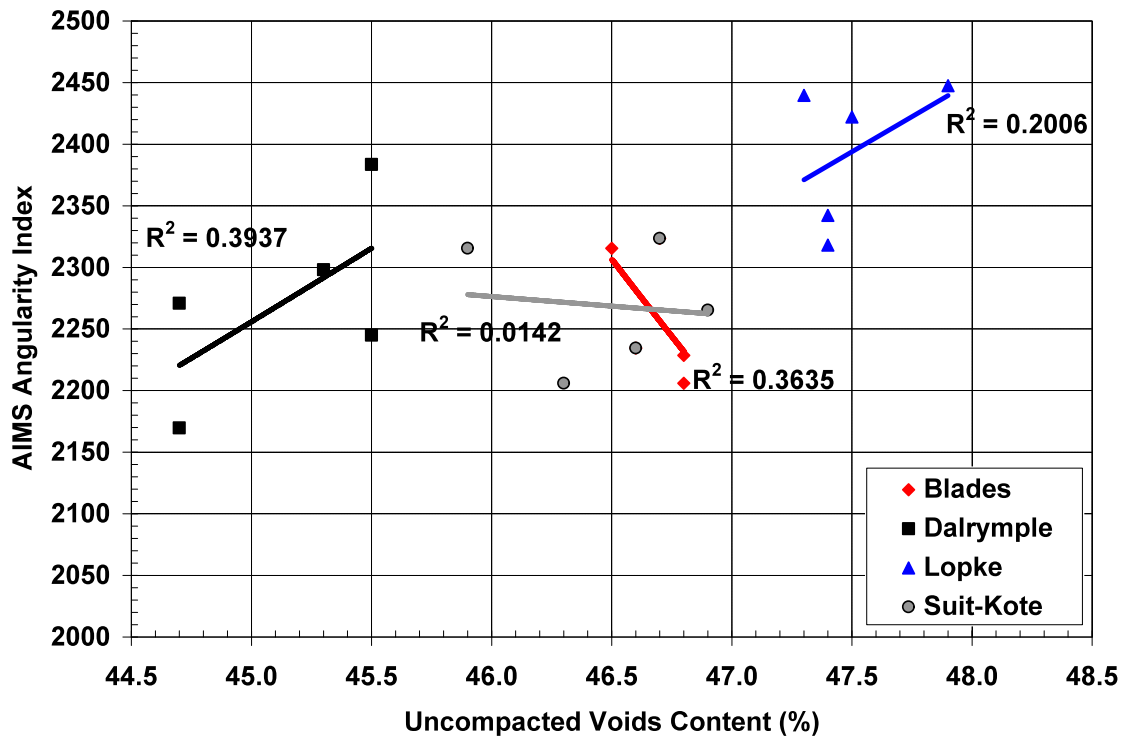
Figure 4.24 – Relationship Between AIMS Angularity Index and Uncompacted Voids Content for Each Independent Gravel Source
