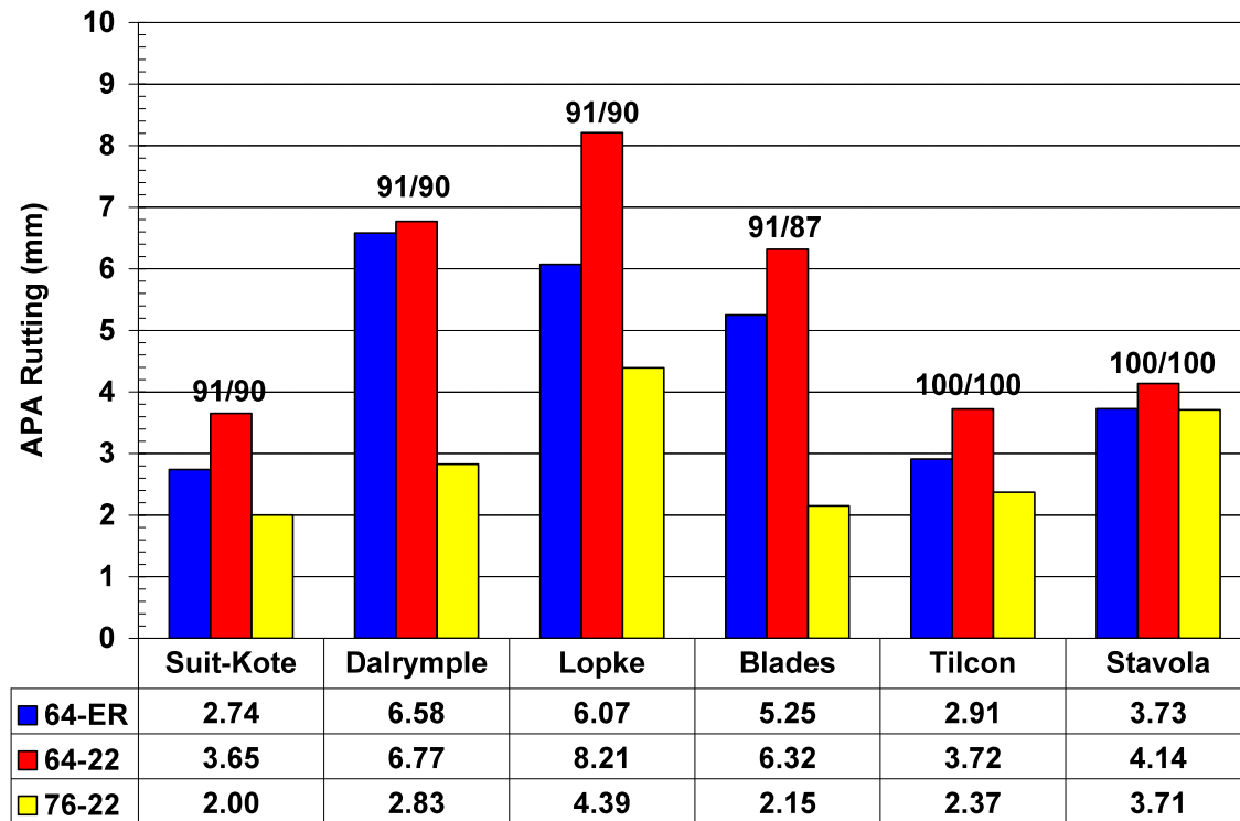
Figure 6.6 – Asphalt Pavement Analyzer Results for 91% One Face Fractured Count
