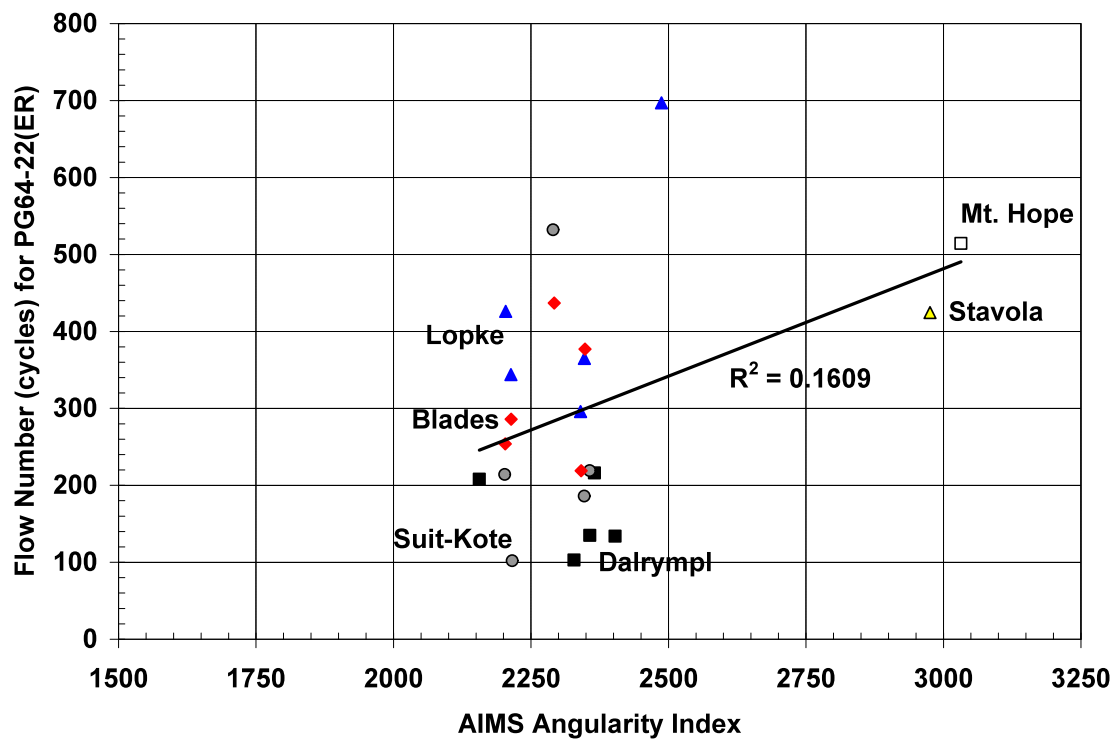
Figure 6.35 – AIMS Angularity Index vs Flow Number for the PG64-22(ER) Asphalt Binder
