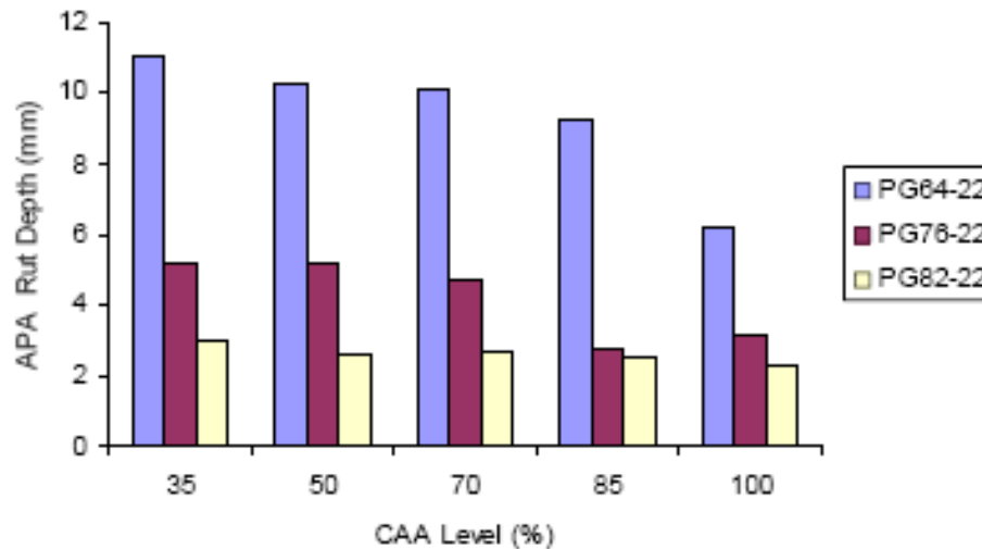
Figure 2.5 – APA Rutting Results of Test Specimens with Varying PG Grade and Coarse Aggregate Angularity (After Huang et al., 2008)
