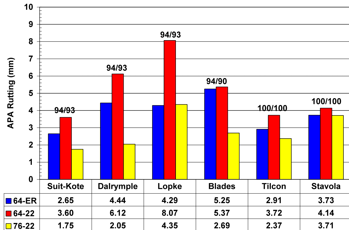
Figure 6.5 – Asphalt Pavement Analyzer Results of 94% One Face Fractured Count
