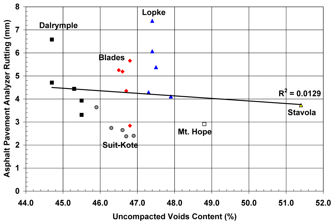
Figure 6.14 – Asphalt Pavement Analyzer Rutting for All Mixtures vs Uncompacted Voids Content – PG64-22 (ER)
