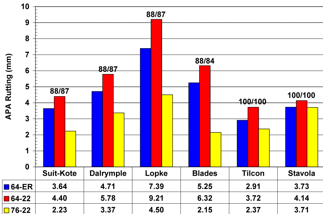
Figure 6.7 – Asphalt Pavement Analyzer Results for 88% One Face Fractured Count
