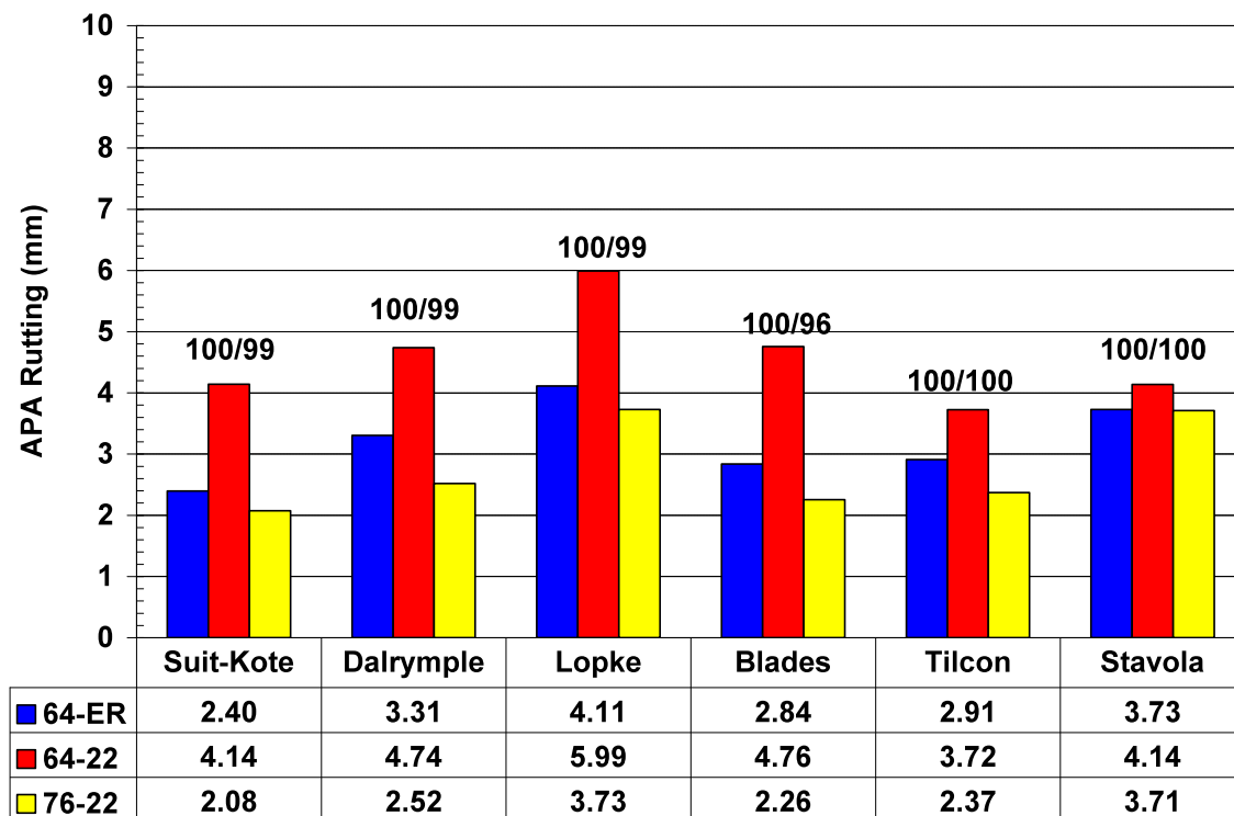
Figure 6.3 – Asphalt Pavement Analyzer Results of Crushed Gravel and Crushed Stone Sources
