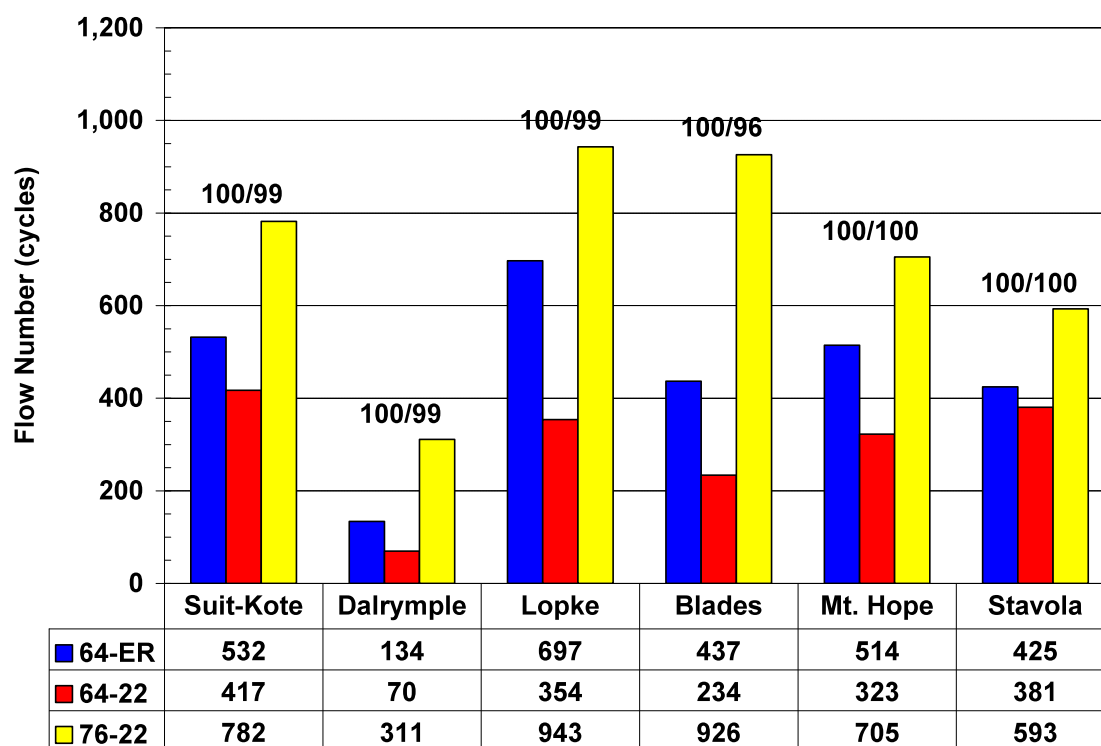
Figure 6.21 – Average Flow Number Results for Baseline Aggregates
