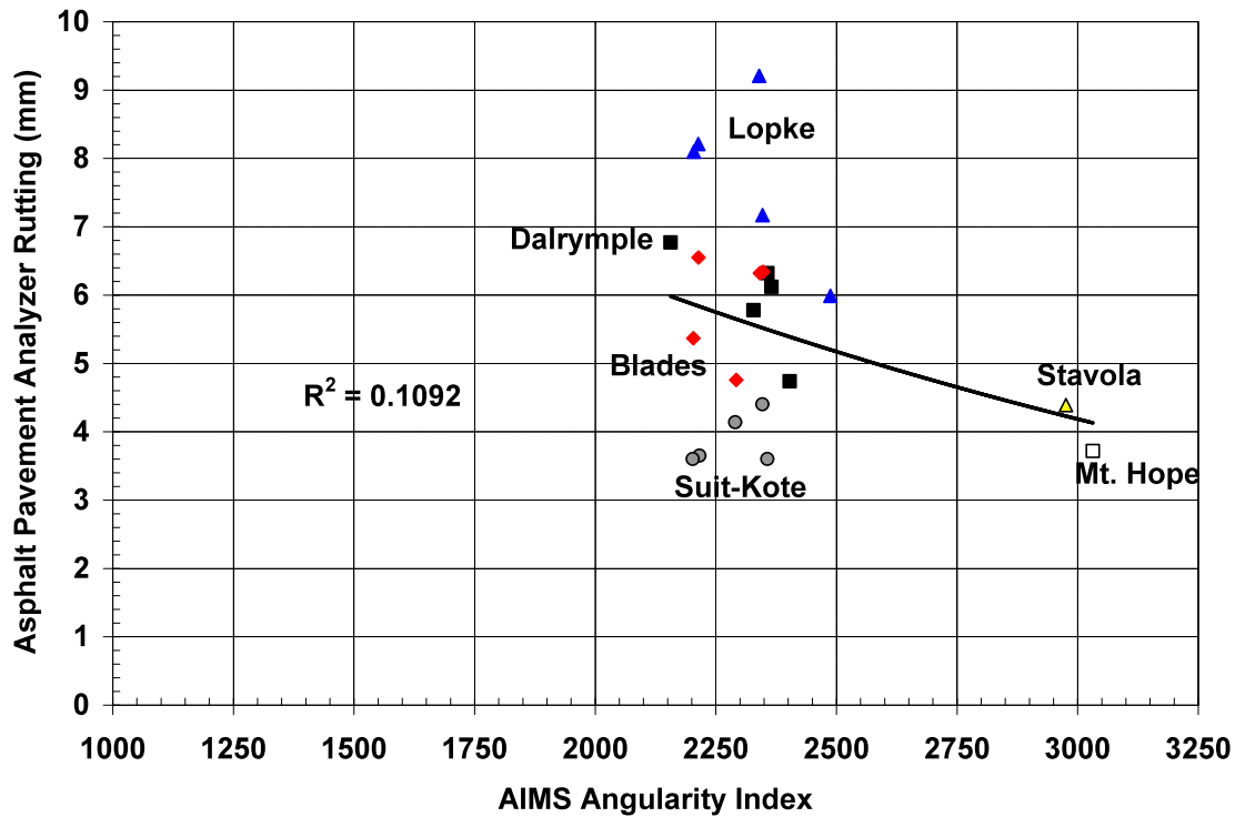
Figure 6.17 – Asphalt Pavement Analyzer Rutting for All Mixture vs AIMS Angularity Index – PG64-22 Asphalt Binder
