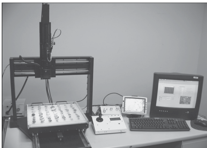
Figure 2.1 – Aggregate Imaging System (AIMS) and Its Components
