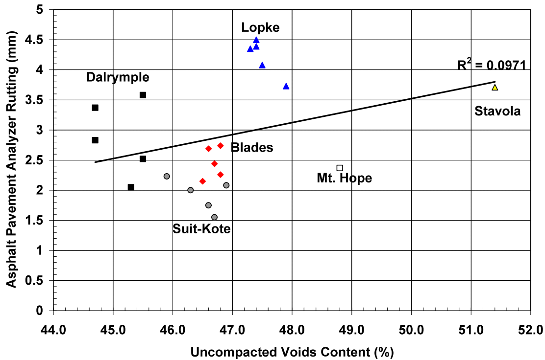
Figure 6.15 – Asphalt Pavement Analyzer Rutting for All Mixtures vs Uncompacted Voids Content – PG76-22 Asphalt Binder
