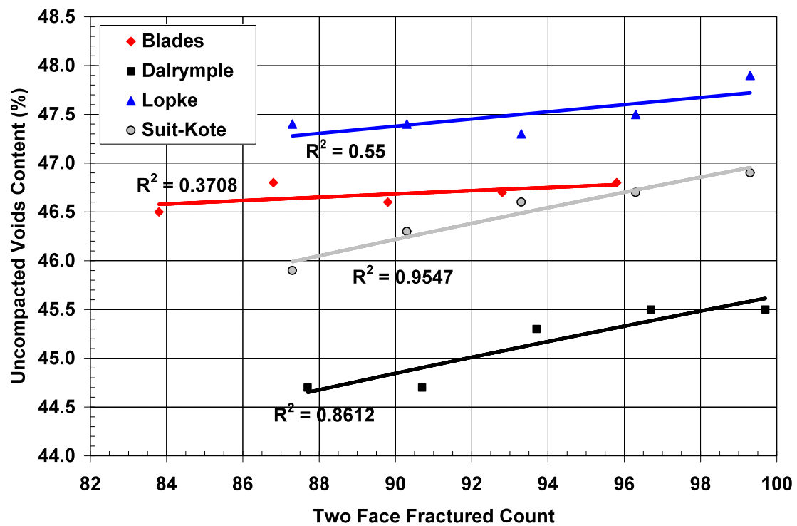
Figure 4.16 – Gravel Source Relationship Between Uncompacted Voids Content and Two-Face Fractured Count
