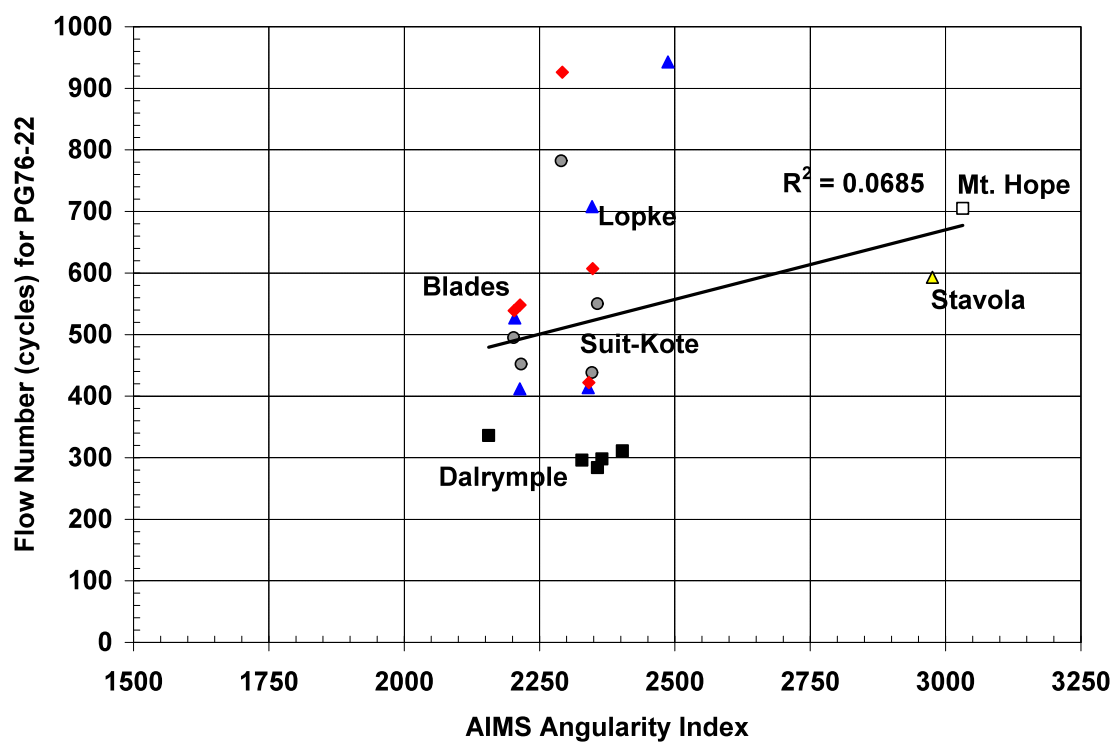
Figure 6.36 – AIMS Angularity Index vs Flow Number for the PG76-22 Asphalt Binder
