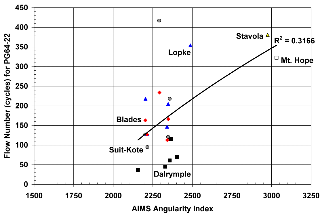
Figure 6.34 – AIMS Angularity Index vs Flow Number for the PG64-22 Asphalt Binder
