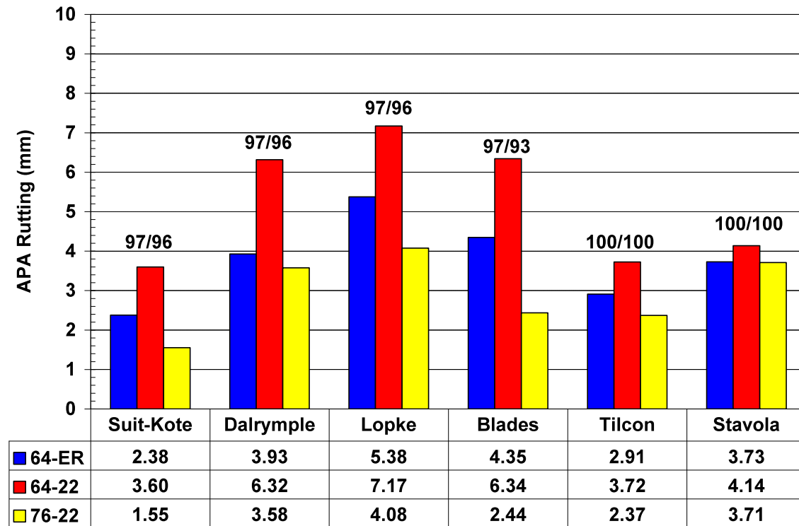
Figure 6.4 – Asphalt Pavement Analyzer Results of 97% One Face Fractured Count
