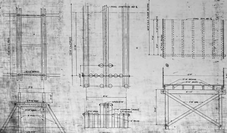
SECTION H-H SECTION J-J CROSS SECTION OF PIERS
