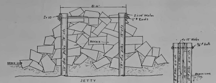
JETTY SECTION "D-D" SCALE: 1/4"=1'-0"
