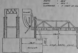
LIFT BRIDGE AT STA SC-6 NOT TO SCALE
