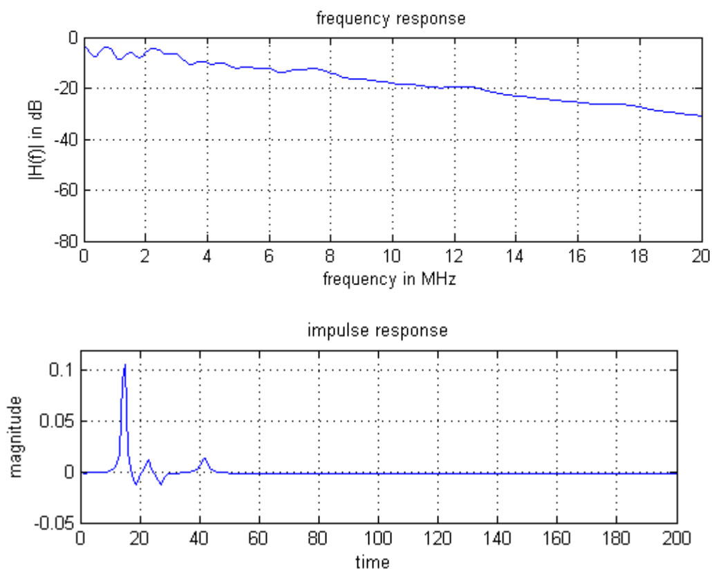
Figure 6.9 Frequency and impulse responses of Reference Channel 1 (RC1).
