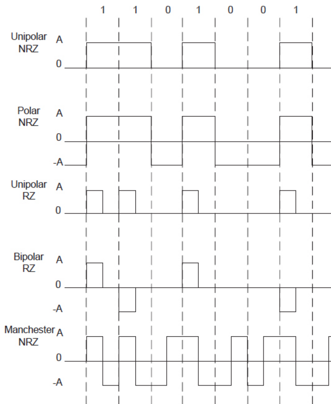
Figure 2.1 Comparison of Digital Line Code waveforms.
