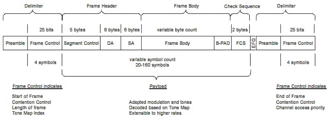
Figure 5.10 PowerPacket Frame Format [Courtesy: Intellon] [68].
