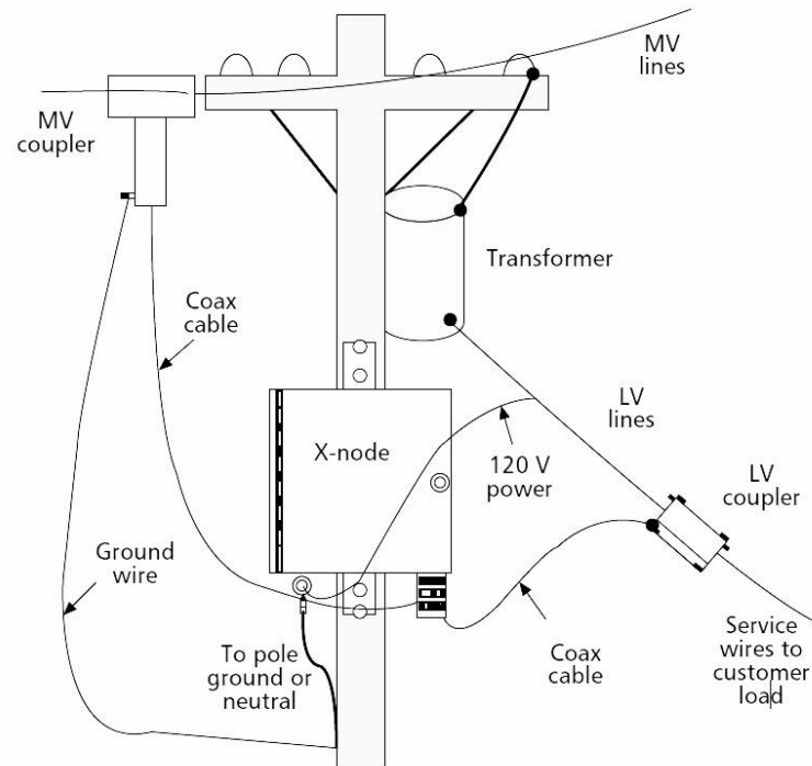
Figure 3.3 Transformer bypass path [8].
