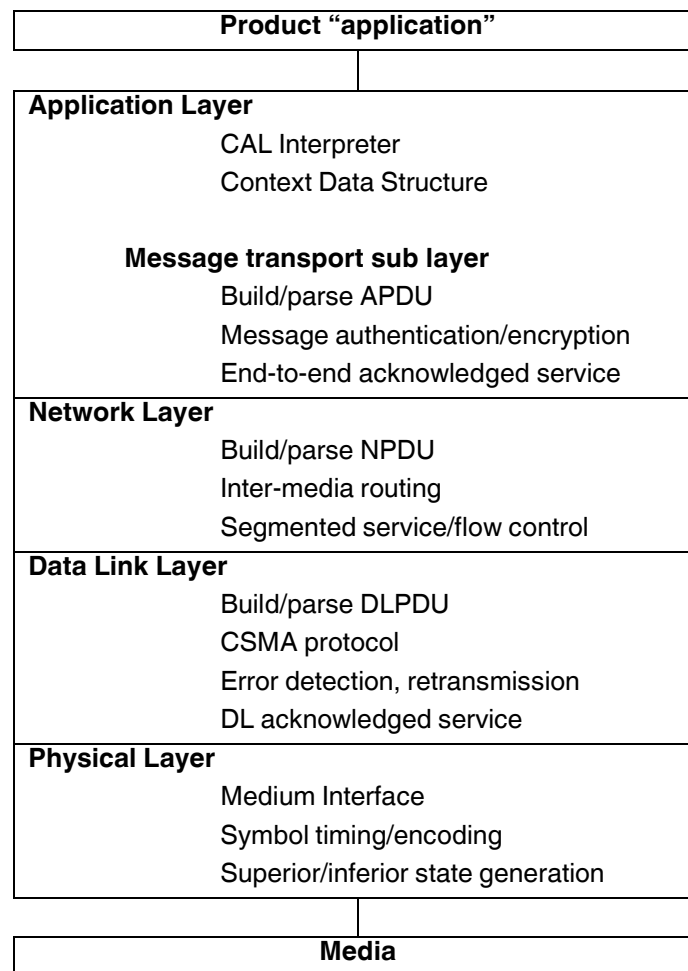
Figure 5.4 CEBus protocol "stack".
