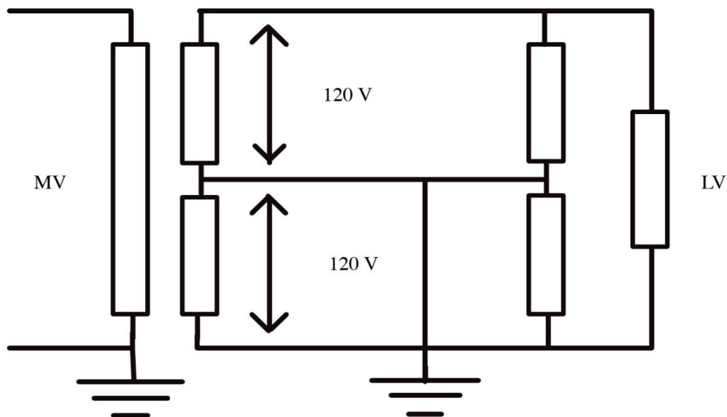
Figure 1.3 U.S. split phase system with MV/LV transformer and loads.
