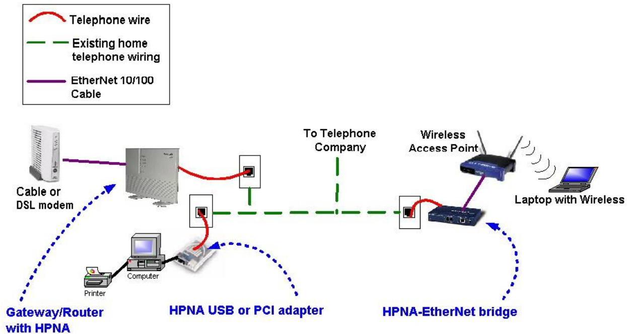
Figure 3.1 Typical HomePNA Network [Courtesy: HomePNA].
