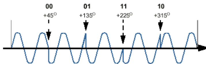
Figure 2.5 A PSK modulated signal having four distinct states.
