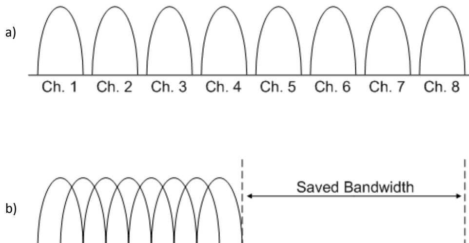
Figure 4.5: a) The frequency spectrum of eight channels shown utilizing frequency division multiplexing. Parallel transmitters are employed in which guard bands are placed between sub-carriers. b) The frequency spectrum of OFDM is shown where sub-channels are orthogonal to the adjacent channel. The percentage of bandwidth used to transmit the same data is reduced by 50%.
