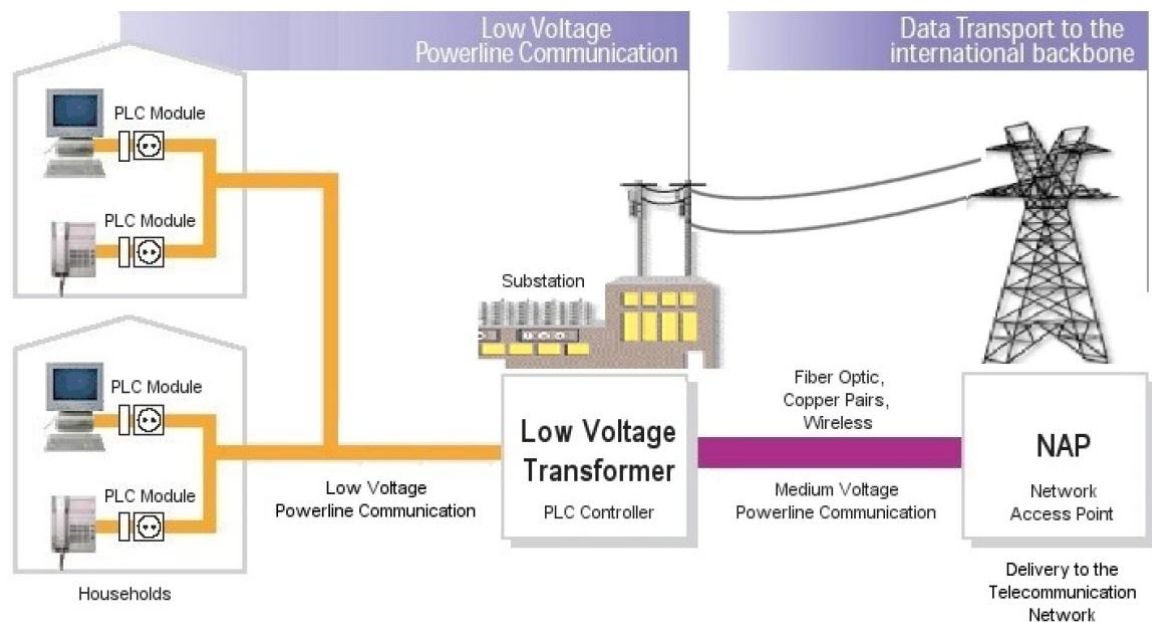
Figure 3.5 Powerline In-House Technology (LV) Network [Courtesy: ABB] [74].
