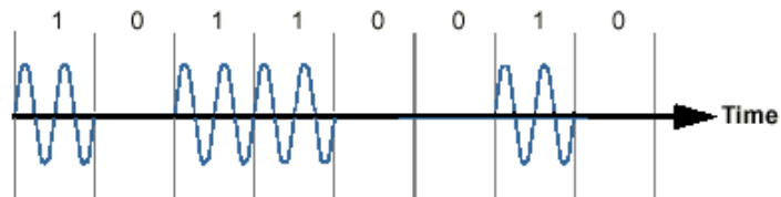
Figure 2.4 On/Off modulation of light in an optical fiber.
