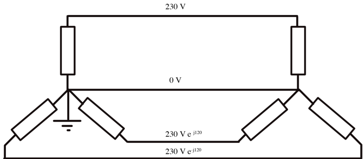
Figure 1.2 European low voltage distribution grid with transformer inductances and loads.
