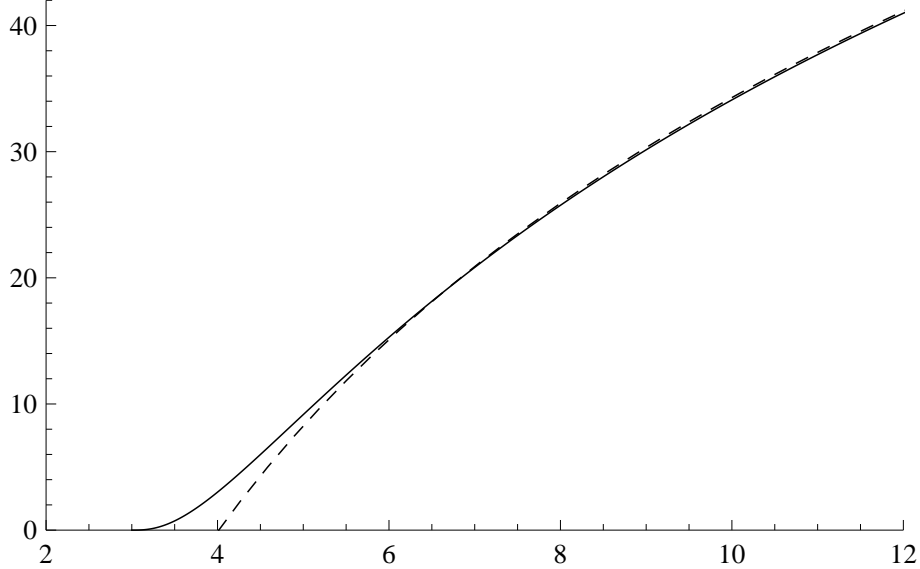
Figure 3.3: Large- E behavior of \sigma_{2 \rightarrow 3}^{(2)}(E) ; the solid line is the result of the numerical evaluation of \sigma_{2 \rightarrow 3}^{(2)}(E) , the dashed line shows the asymptotic form (3.40), which is seen to approximate \sigma_{2 \rightarrow 3}^{(2)}(E) very closely starting from relatively low energies.
