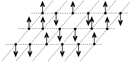
Figure 1.1: A possible spin configuration on a two-dimensional square lattice.
