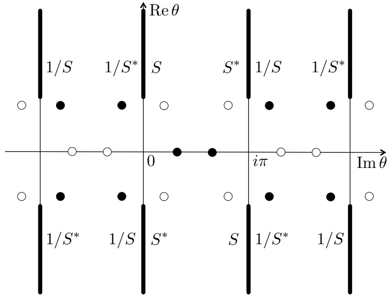
Figure 3.1: Analytic structure of the two-particle scattering amplitude S(\theta) in the complex \theta -plane. The thick lines represent the branch cuts associated with inelastic channels. The values of S(\theta) at different edges of the cuts represent physical S -matrix element S , its complex conjugate S^* , and the inverse values. The bullets \bullet and circles \circ indicate possible positions of poles and zeroes, respectively. Poles located on the imaginary axis within the physical strip 0 < \text{Im } \theta < \pi correspond to stable particles, poles in the mirror strip -\pi < \text{Im } \theta < 0 are associated with resonance scattering states.
