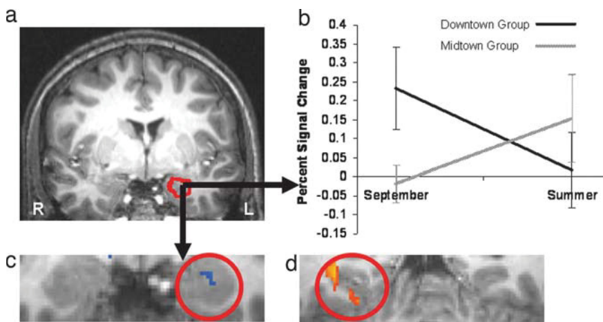
Fig. 2. Blood oxygen level-dependent (BOLD) response and proximity to the WTC. (a) Coronal slice of the structurally defined left amygdala (outlined in red) that includes the peak active voxel. (b) Mean percentage signal change from the peak active voxel in the left amygdala, revealing a two-way interaction of trial type (9/11 vs. summer) \times group (Downtown vs. Midtown). (c and d) ANCOVA contrasting activation during 9/11 trials vs. summer trials, with participants' distance from the WTC as a covariate, in voxels within the structurally defined amygdala (c) and posterior parahippocampal cortex (d). Warm colors indicate positive correlation ( r_{pb} < 0.02 , uncorrected), and cool colors indicate negative correlation ( r_{pb} < 0.02 , uncorrected). Participants who were closer to the WTC showed decreased activation in the posterior parahippocampal cortex and increased activation in the amygdala bilaterally during retrieval of 9/11 memories relative to summer memories.
