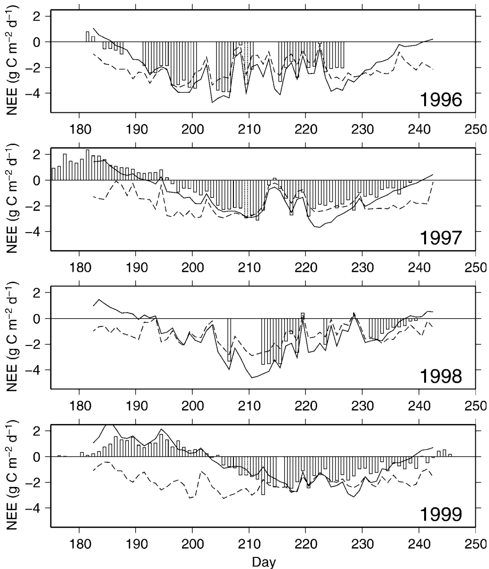
FIGURE 7. Daily net ecosystem exchange during the period 1996–1999. The bars represent measurements. The solid line shows the modeled NEE based on a leaf area index and V_{cmax} that varied individually for each year. The dashed line shows the modeled NEE based on a constant LAI and V_{cmax} where the values of LAI and V_{cmax} are the average values from the 4-yr period.
