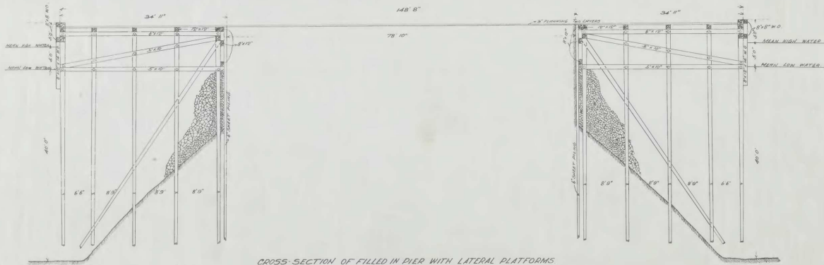
CROSS SECTION OF FILLED IN PIER WITH LATERAL PLATFORMS
