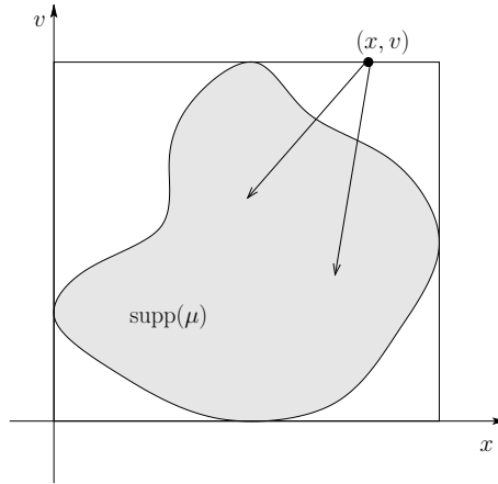
FIG. 4.1. Vector field \xi[\mu]
