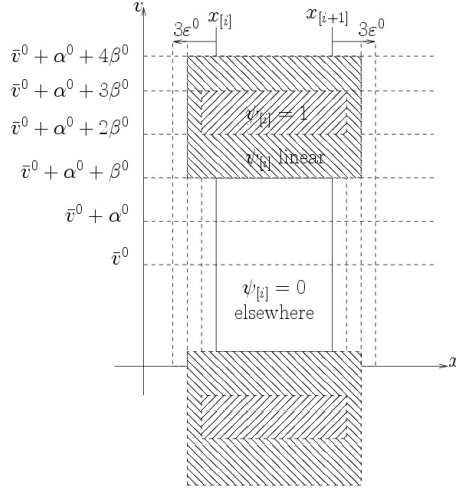
FIG. 4.2. Definition of \psi_{[i]} .
