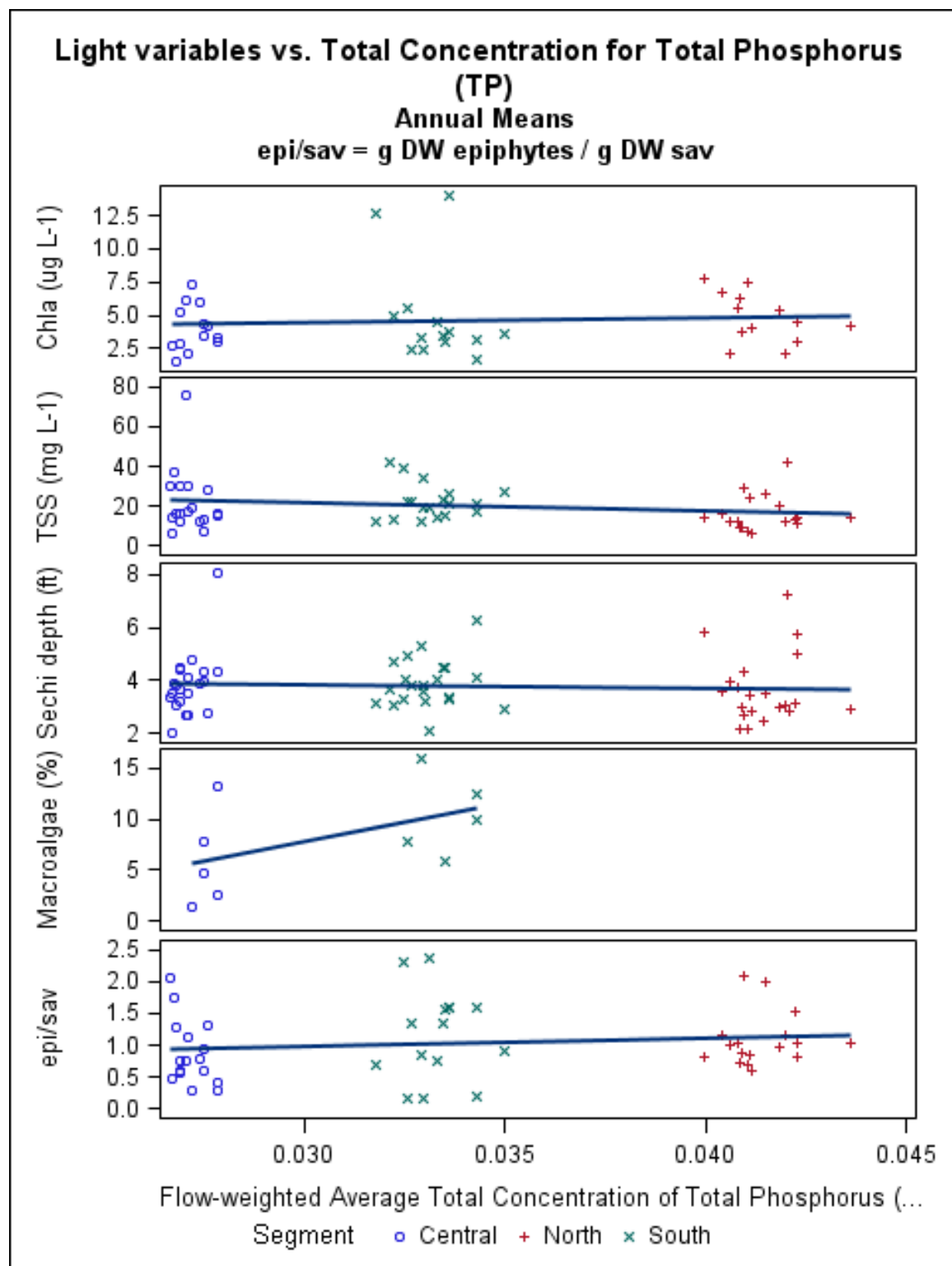
Figure 3 - 6 Light indicators vs. flow-weighted average total concentration of total phosphorus ( \text{mg L}^{-1} ).
