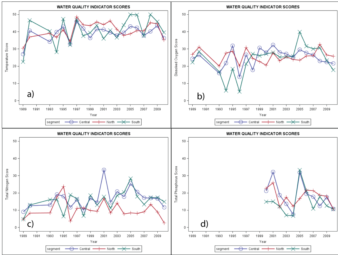
Figure 3 - 49 Scores for Water Quality indicators: (a) temperature, (b) dissolved oxygen, (c) total nitrogen, (d) total phosphorus.
