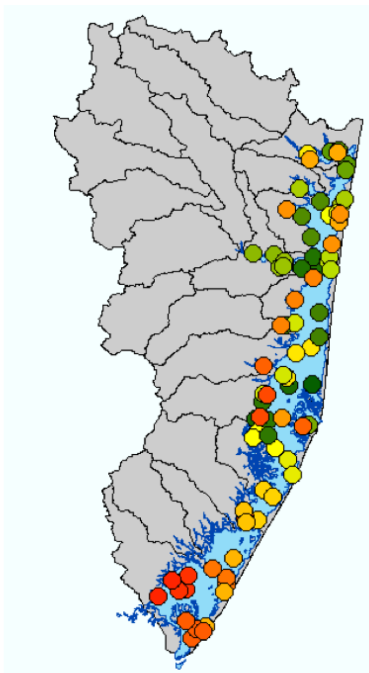
Figure 2 - 25 Benthic invertebrate sampling stations (2001) of the USEPA Regional Monitoring and Assessment Program for the BB-LEH Estuary.
