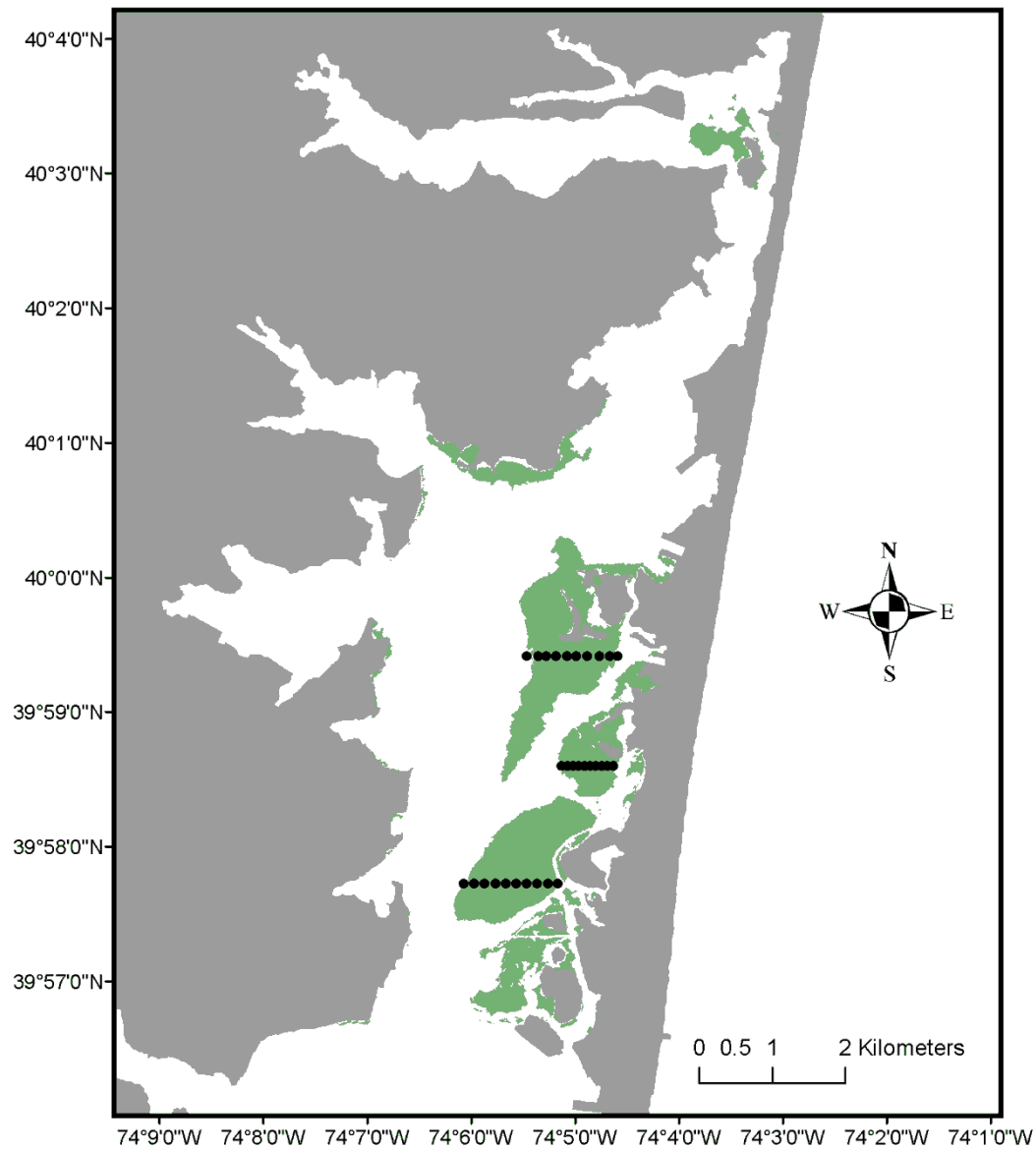
Figure 1 - 10 Seagrass transects established in the north segment of the BB-LEH Estuary for SAV sampling in 2011.
