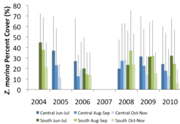
Figure 2 - 17 Mean eelgrass percent cover in the central and south segments of the BB-LEH during the spring-fall sampling periods from 2004 to 2010.
