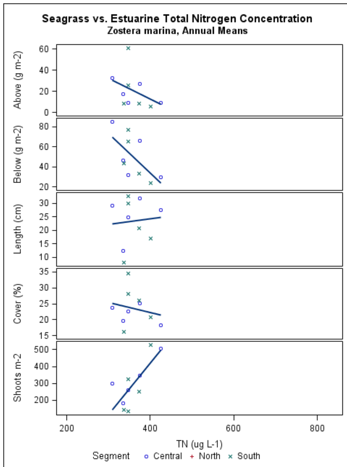
Figure 3 - 32 Seagrass indicators vs estuarine total nitrogen
