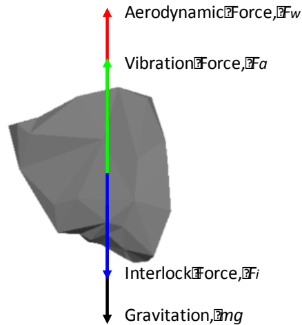
Figure 4.1 Schematic ballast flying mechanic equilibrium (Jing et al., 2012)
