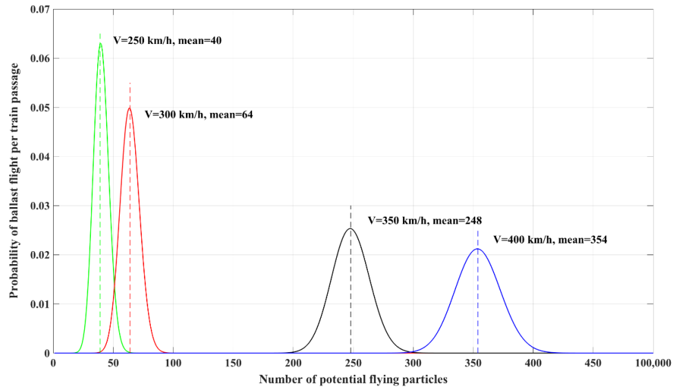
Figure 4.6 Distribution of the number of ballast flight per train passage (center line of track, P1 position)
