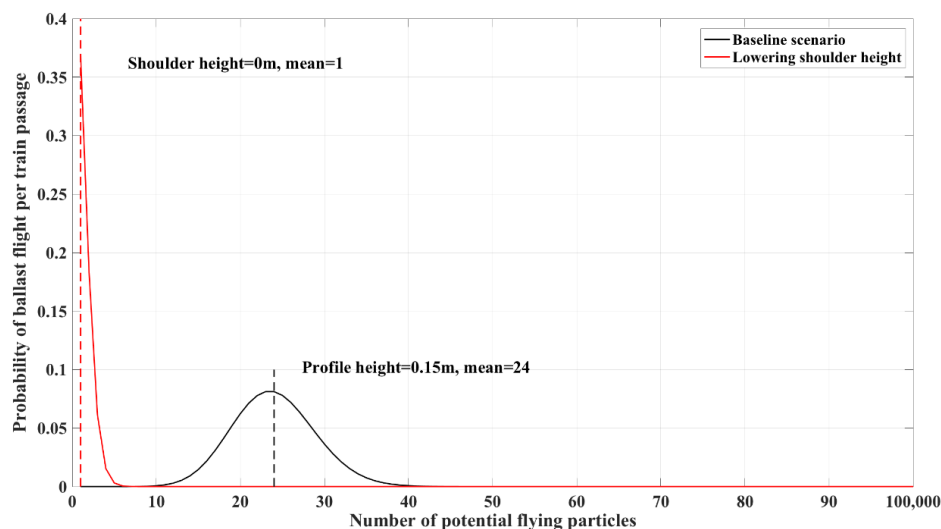
Figure 4.8 Number of ballast flight per train passage, measured position: P4
