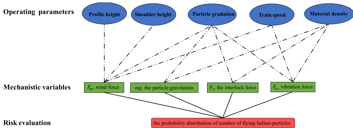
Figure 4.2 The relationship between operating variables, mechanistic variables and flying ballast risk
