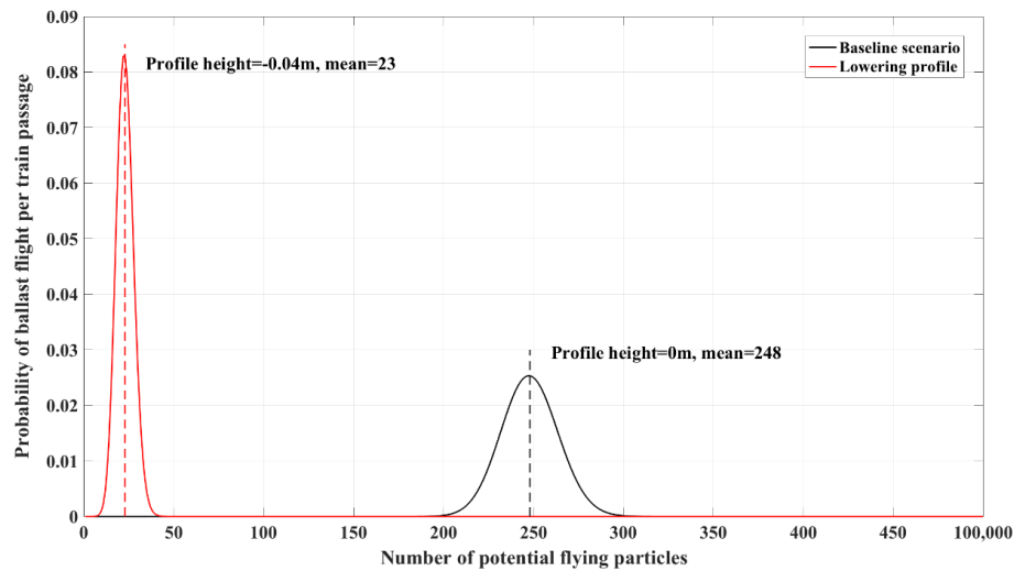
Figure 4.7 Distribution of the number of ballast flight per train passage for track centerline, P1
