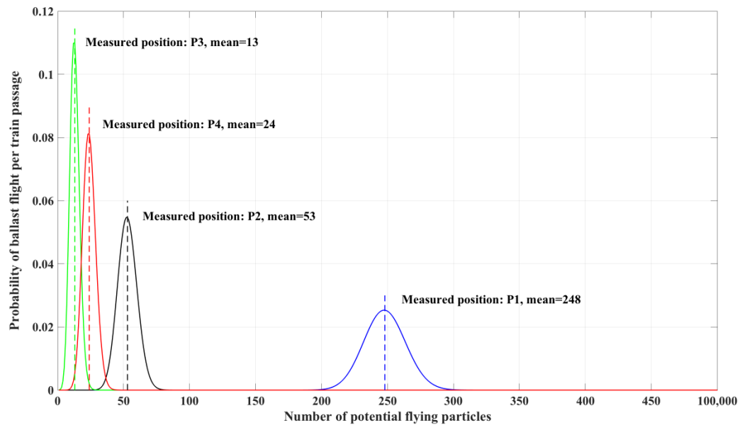
Figure 4.5 Probabilistic distribution of the number of ballast flight per train passage, V_{train} = 350 \text{ km/h}
