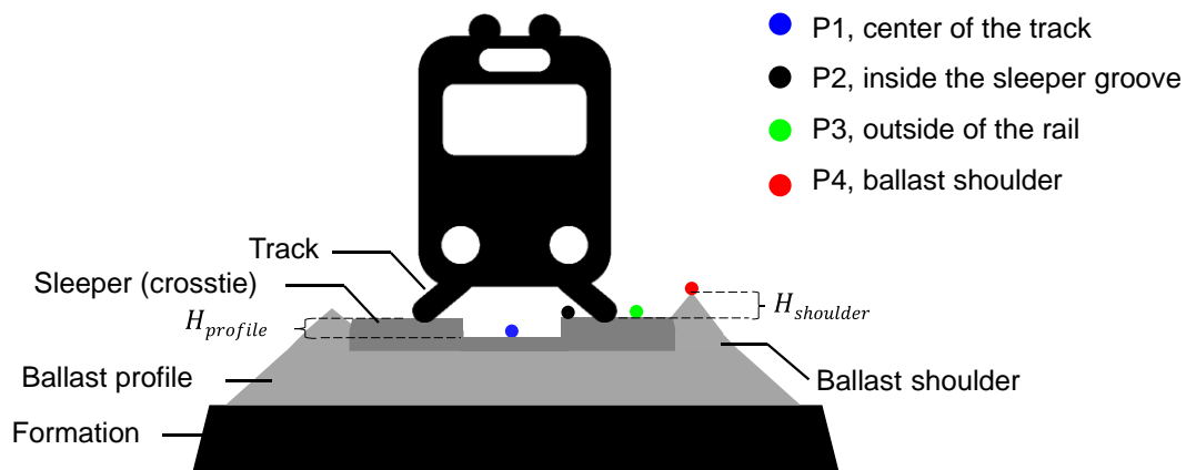
Figure 4.4 Schematic diagram of track model and the points of interest on the track
