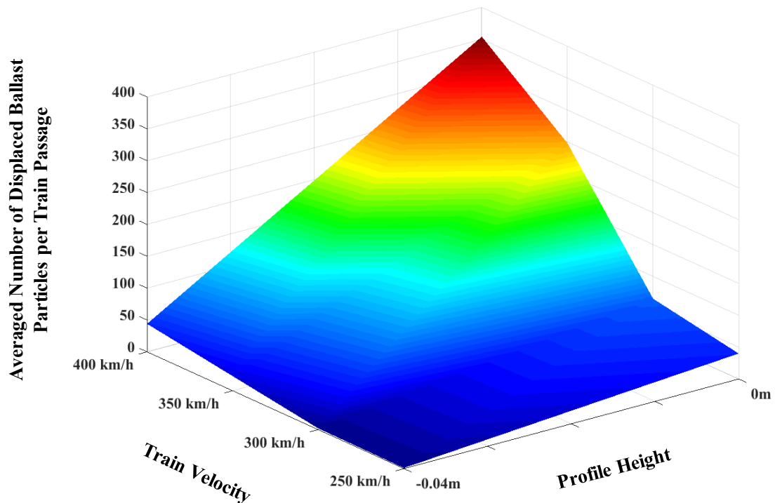
Figure 4.10 Effect of ballast profile and speed on flying ballast risk (track centerline, P1)
