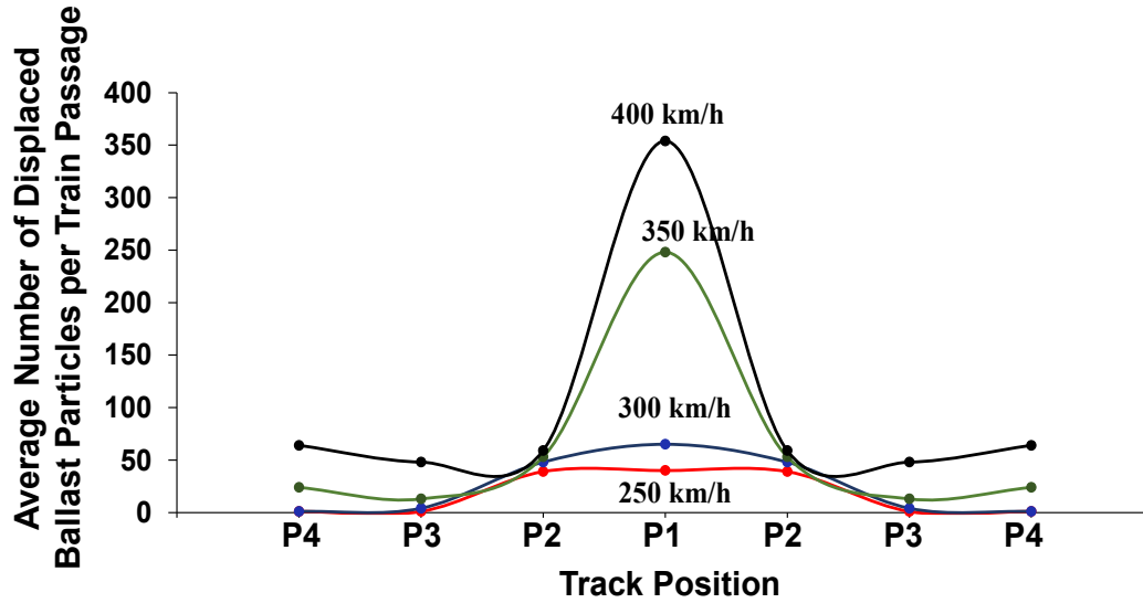
Figure 4.9 Flying ballast risk (mean number of flying ballast particles) by track position and speed on the studied HSR segment, ballast profile is at the top of a sleeper, ballast shoulder height is 0.15 m
