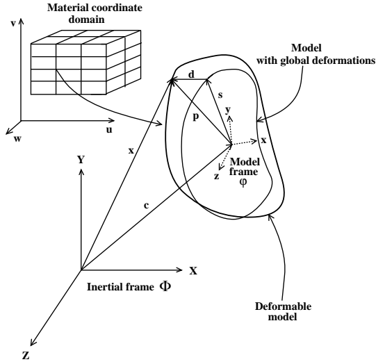
Figure 7: Geometry of Deformable Models
