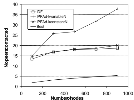
Figure 6. Number of peers contacted as a function of the community size when k is kept constant at 20. IPF Ad-k variable N is TFxIPF with the adaptive stopping heuristic. IPF Ad-k constant N is TFxIPF with a stopping heuristic that is only a function of k and not of community size. All these plots were obtained using a Weibull distribution of documents on the AP89 collection.
