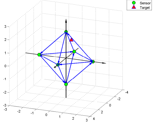
Fig. 10. Figure shows a sensor network where each node is a low cost radar that can sense along the axis it is placed and not the other. The directed edges indicate the directed communication between the nodes. Through cooperative effort the nodes aim to learn location of the target in 3 dimensions.
