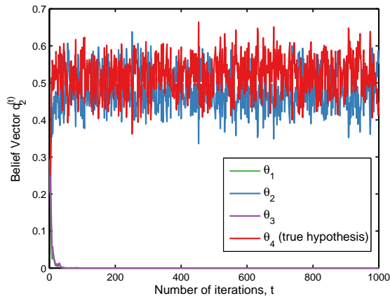
Fig. 4. Figure shows the beliefs of node 2 shown in Figure 1. When the network is not strongly connected node 2 cannot learn \theta_4 .
