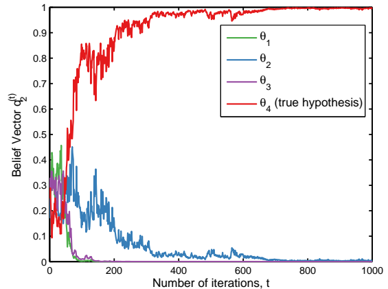
Fig. 2. For the set of nodes described in Figure 1, this figure shows the evolution of beliefs for one instance using the proposed learning rule. Belief of the true hypothesis \theta_4 of node 2 converges to 1 and beliefs of all other hypotheses go to zero.
