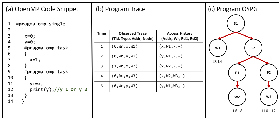
Figure 4.3: (a) OpenMP program snippet with a write-read data race on shared variables x (b) Possible execution trace. (c) The code snippet's OSPG. The code fragment each W-node represents is shown below it.
