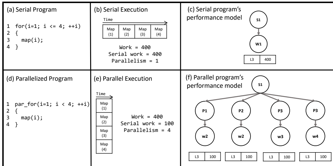
Figure 3.9: A data-parallel for loop executed serially and in parallel. (a) Serial program with data-parallel loop. (b) The serial program's trace. (c) The performance model of the serial program. (d) A parallelized version of the program (e) The parallel program's trace. (f) The performance model of the parallelized program.
