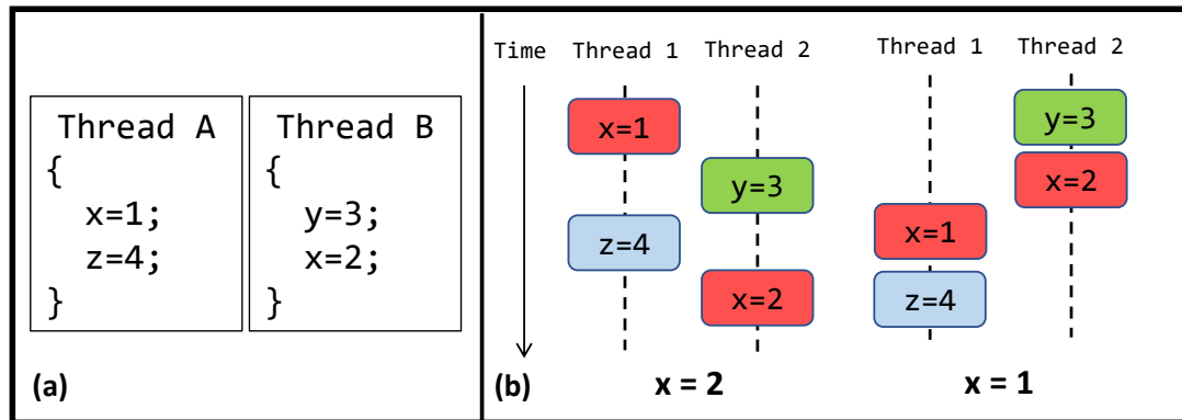
Figure 4.1: (a) Code snippet illustrating a multithreaded program with a data race on shared variable x . (b) Two possible execution traces on a system with two threads.
