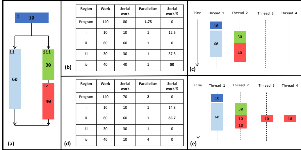
Figure 3.1: An example parallel application and its parallelism profile used to identify which program fragment to optimize first. (a) Illustration of a parallel program’s fragments and the ordering of the fragment’s execution. (b) Parallelism profile of the program. (c) A possible trace of the program when executed on a 4 core machine. (d) The program’s parallelism profile after parallelizing fragment iv by a factor of 4. (e) The optimized program’s trace when executed on a 4 core machine.
