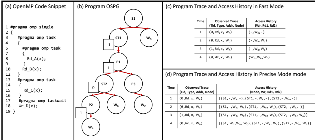
Figure 4.4: Illustration of an example OpenMP program snippet where the use of a constant amount of access history metadata is not sufficient to detect the data race on variable x . (a) OpenMP program snippet. (b) The code snippet's OSPG. (c) Program trace with fast mode's access history metadata management. (d) Program trace using precise mode's access history metadata management.
