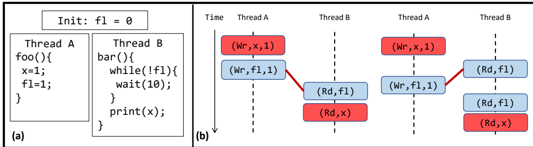
Figure 4.2: (a) Code snippet illustrating a multithreaded program with two apparent data races on shared variables x and fl . (b) Two possible execution traces of the code snippet in (a), illustrating that the data race on variable fl is feasible.
