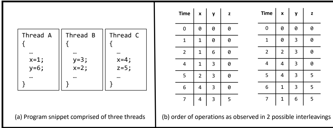
Figure 1.1: (a) Code snippet illustrating 3 threads that write to shared variables x,y, and z. (b) Different interleavings in a multithreaded program may lead to different final values for shared variables. The number of interleavings grows exponentially with thread counts and the operations within each thread. The example illustrates two possible traces that produce different results.
