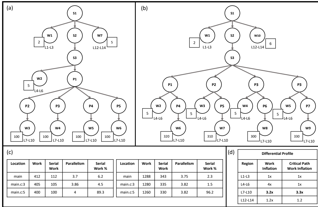
Figure 3.11: (a) The performance model of the single thread execution of the program in Figure 3.10)(c). (b) The performance model of the parallel execution of the program in Figure 3.10)(c) with four worker threads.
